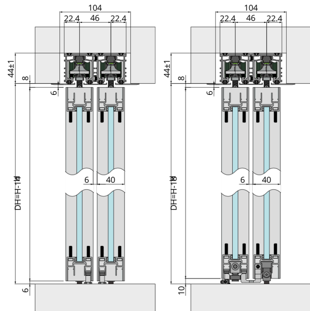
Overlap 2 Doors
