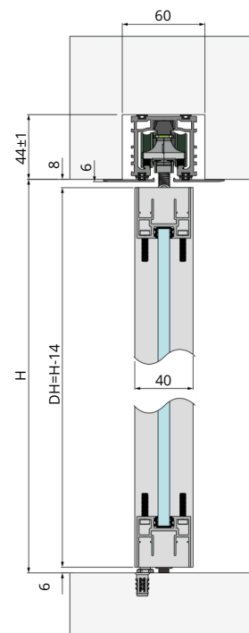
CONCEALED MOUNTING
