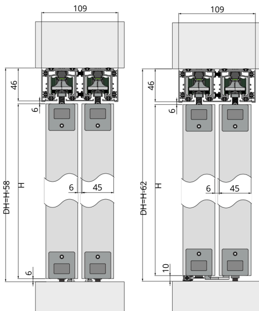
Overlap 2 Doors
