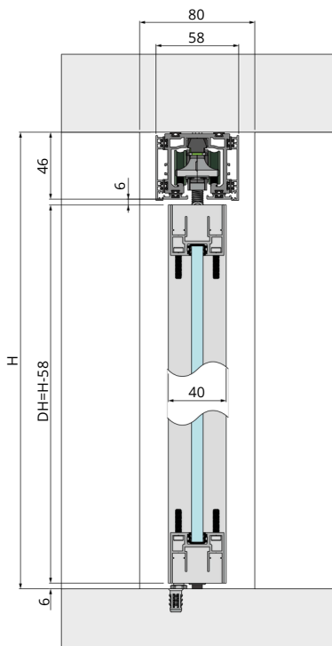
SURFACE MOUNTING
