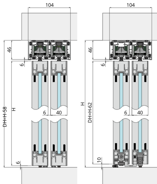
Overlap 2 Doors
