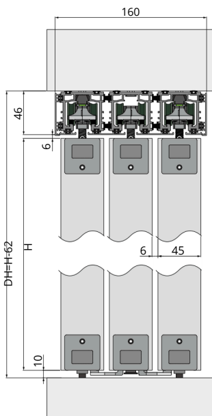
SURFACE MOUNTING
