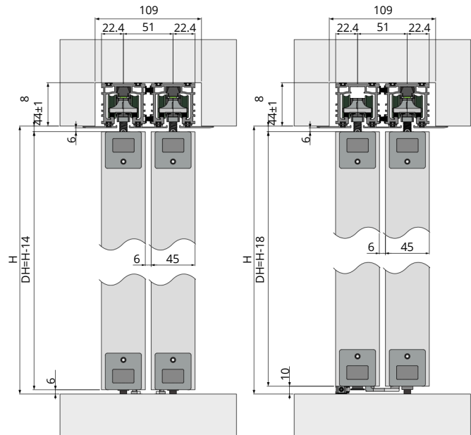
Overlap 2 Doors
